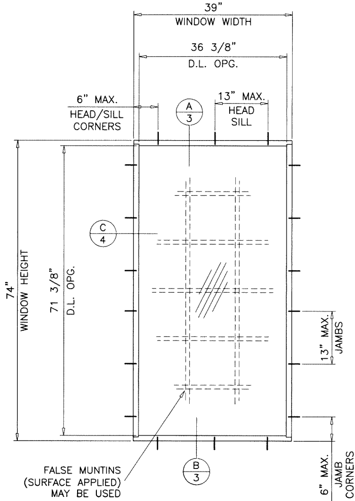
TYPICAL ELEVATIONS (TESTED UNITS)
